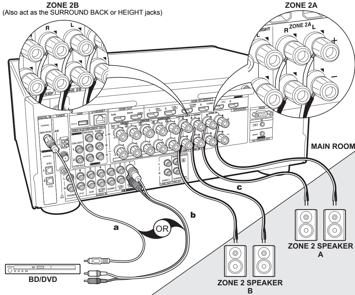
a Digital coaxial cable, b Analog audio cable, c Speaker cable
