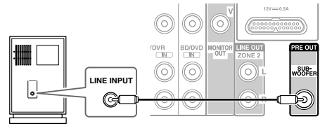
Powered subwoofer
